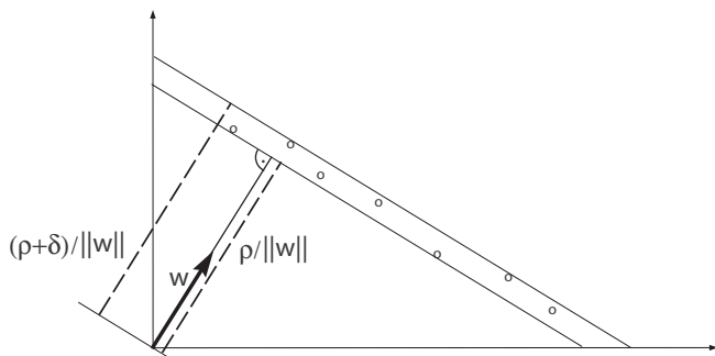
Figure 1: The geometric set-up for the slab SVM.
