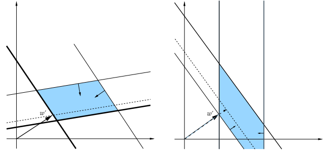
Figure 3: The lower (non-moving) constraints are shown by thick solid lines and the upper (moving) constraints are shown by thin solid lines. On the left: when the moving constraint hits w' this constraint becomes binding (gain event) and the solution is no longer stationary. On the right: once the moving constraint becomes orthogonal to w' we lose the non-moving constraint (lose event).
